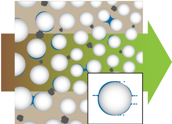
Traditional Tube Cross Section: Typical void spaces to capture liquid and solid particulates. Conventional pathways for standard gas flow.
