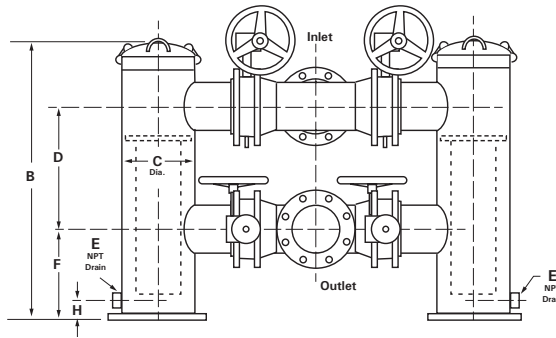
950 B 8"- 12" quick open cover
