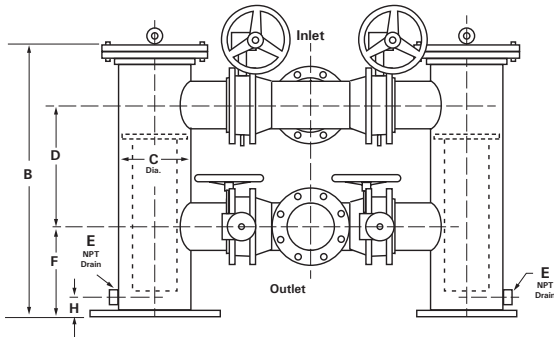
950 B 8"- 12" bolted cover
