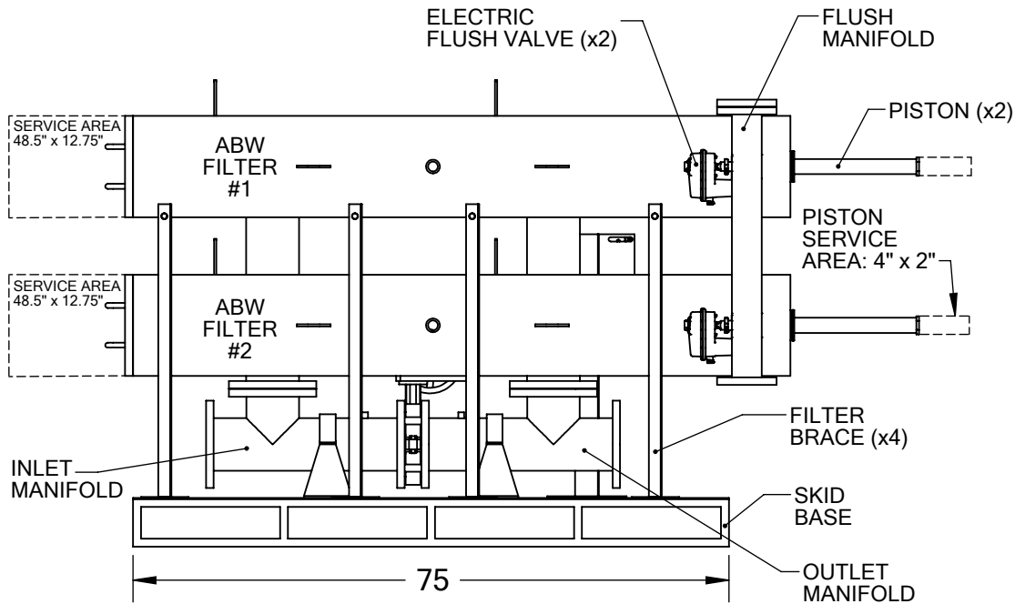
SIDE VIEW
